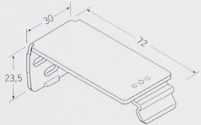
Extensions Face Fix Bracket
