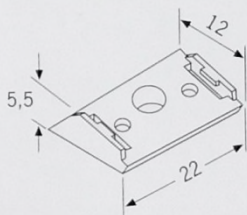
Angle Fixing 15°
