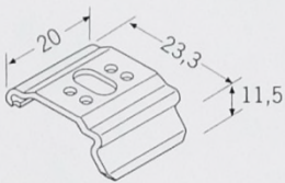
Top Fix Bracket
