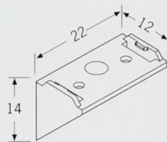
Angle Fixing 45°
